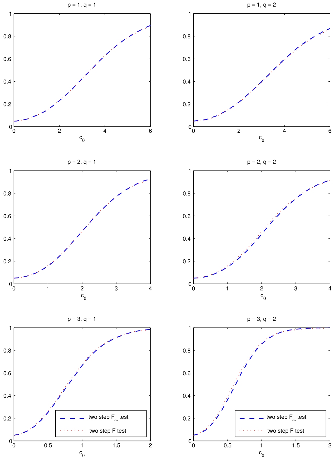
Fig. 4. Size-adjusted power of two-step 5% F_\infty and F tests based on the series LRV estimator under the AR design with \rho = 0.5 and T = 100 .
