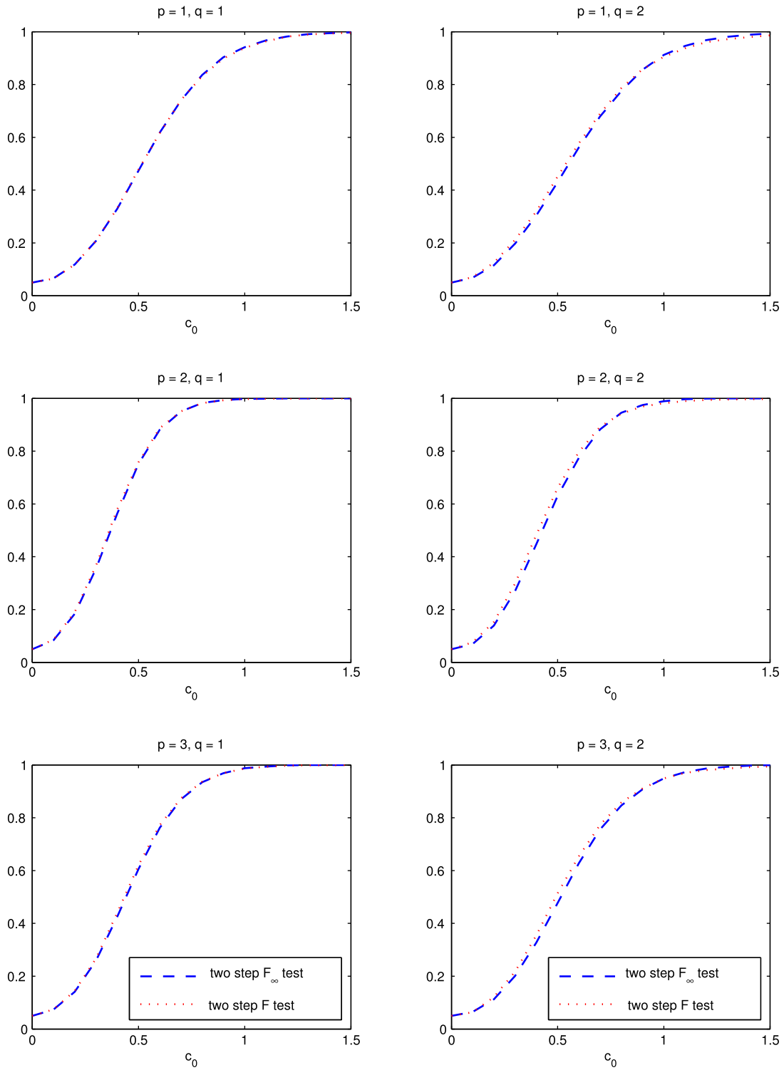
Fig. 5. Size-adjusted power of two-step 5% F_\infty and F tests based on the series LRV estimator under the centered MA design with L = 9 and T = 100 .
