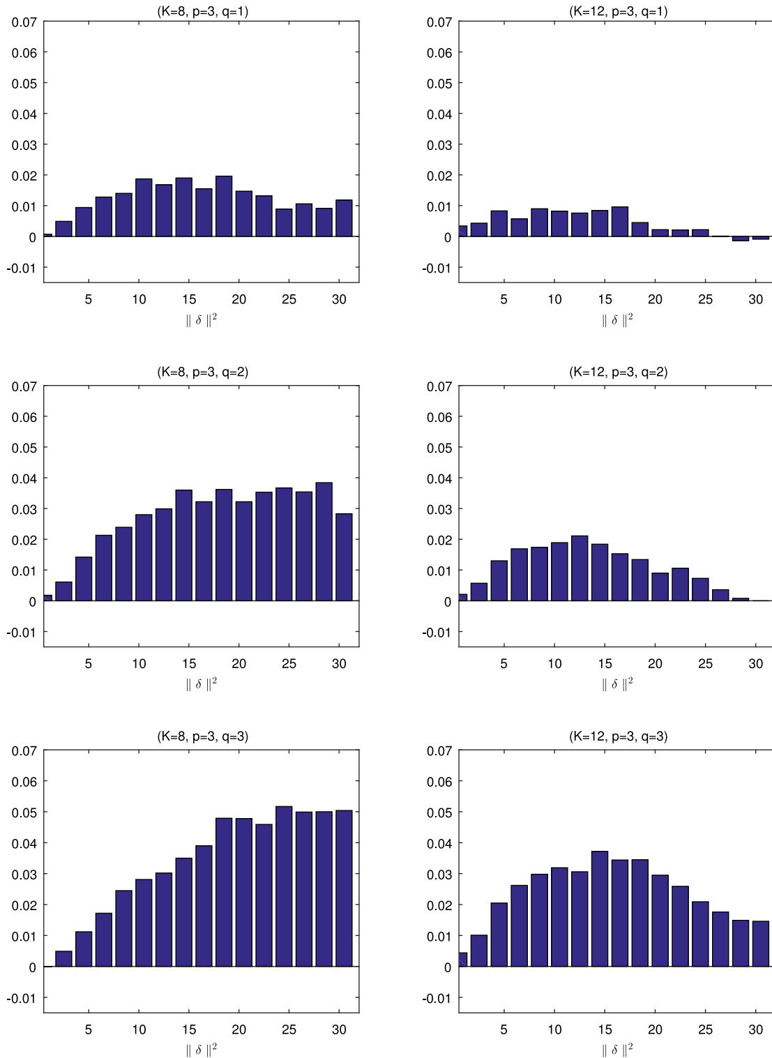
Fig. 1. Difference of the asymptotic local power between the nonstandard F_\infty test and the standard F test \pi^\epsilon(\cdot) - \pi(\cdot) for K = 8, 12, q = 1, 2, 3 , and p = 3 .
