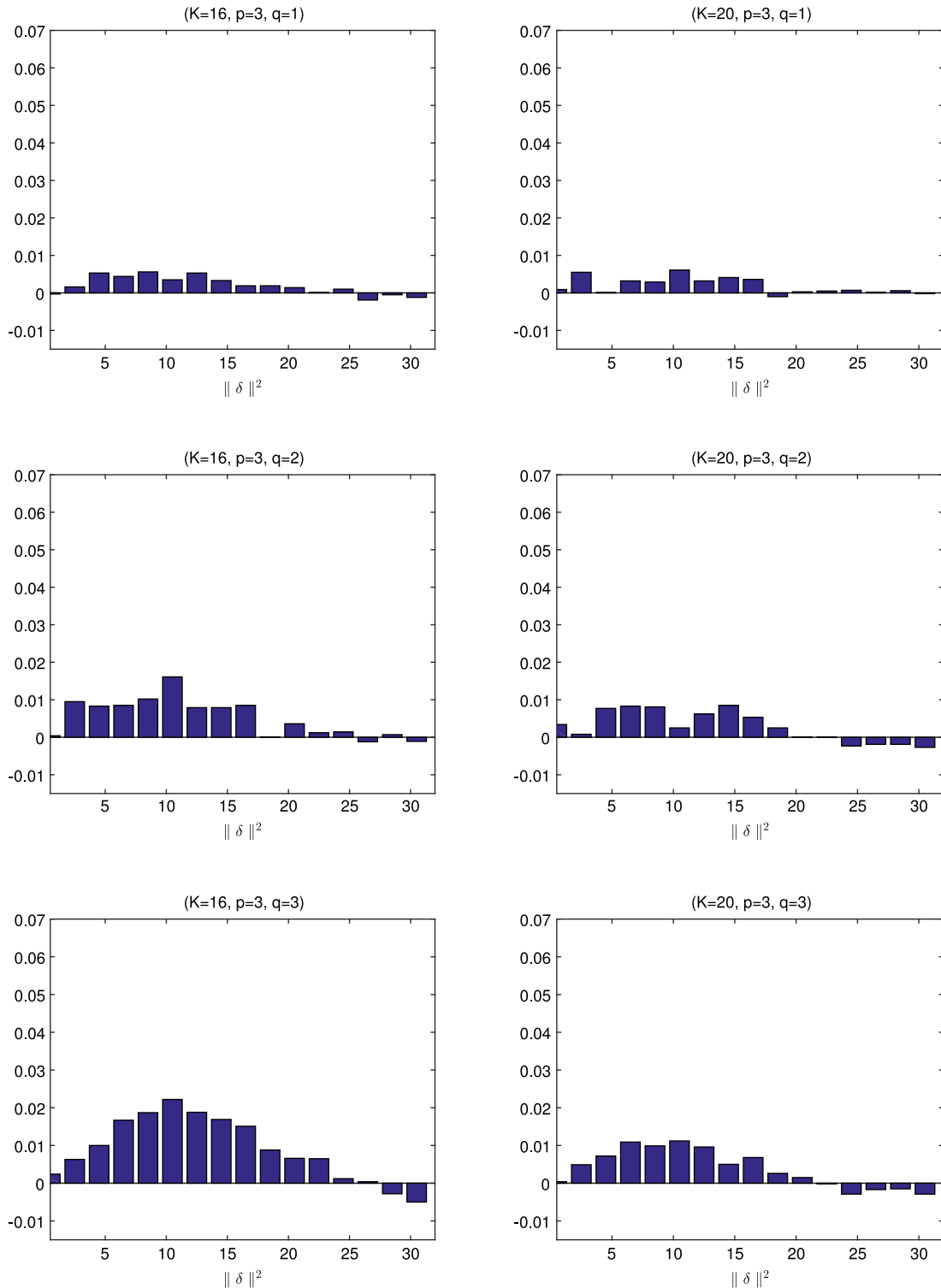
Fig. 2. Difference of the asymptotic local power between the nonstandard F_\infty test and the standard F test \pi^c(\cdot) - \pi(\cdot) for K = 16, 20, q = 1, 2, 3 , and p = 3 .
