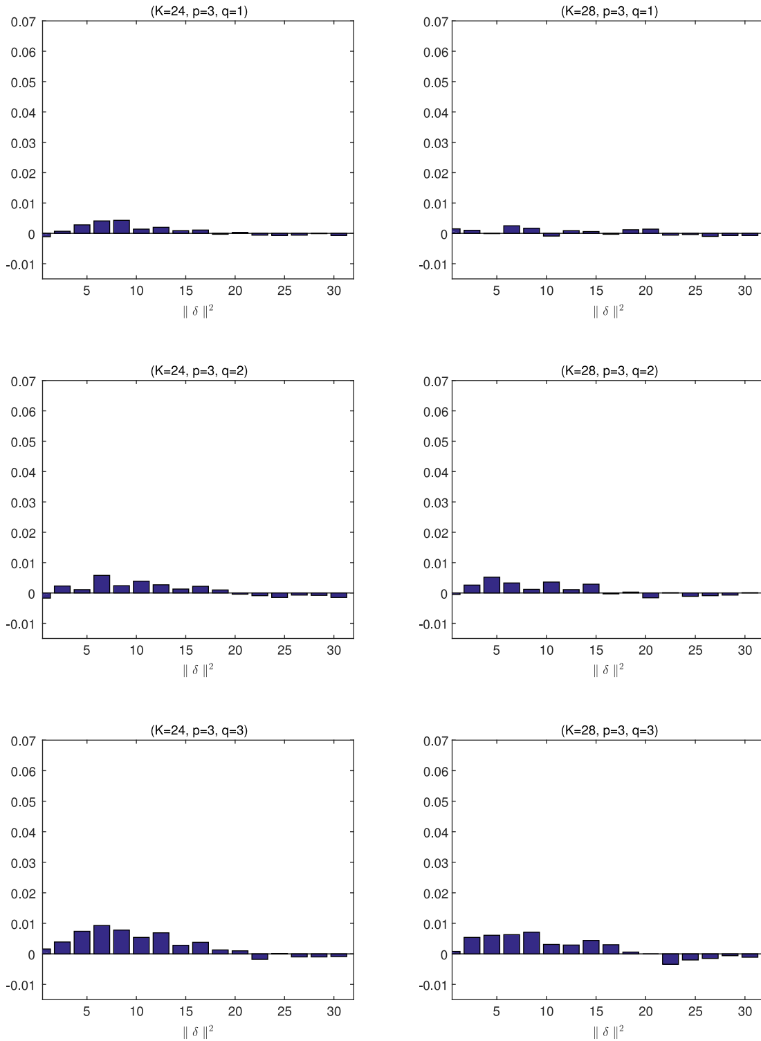
Fig. 3. Difference of the asymptotic local power between the nonstandard F_\infty test and the standard F test \pi^c(\cdot) - \pi(\cdot) for K = 24, 28, q = 1, 2, 3 , and p = 3 .
